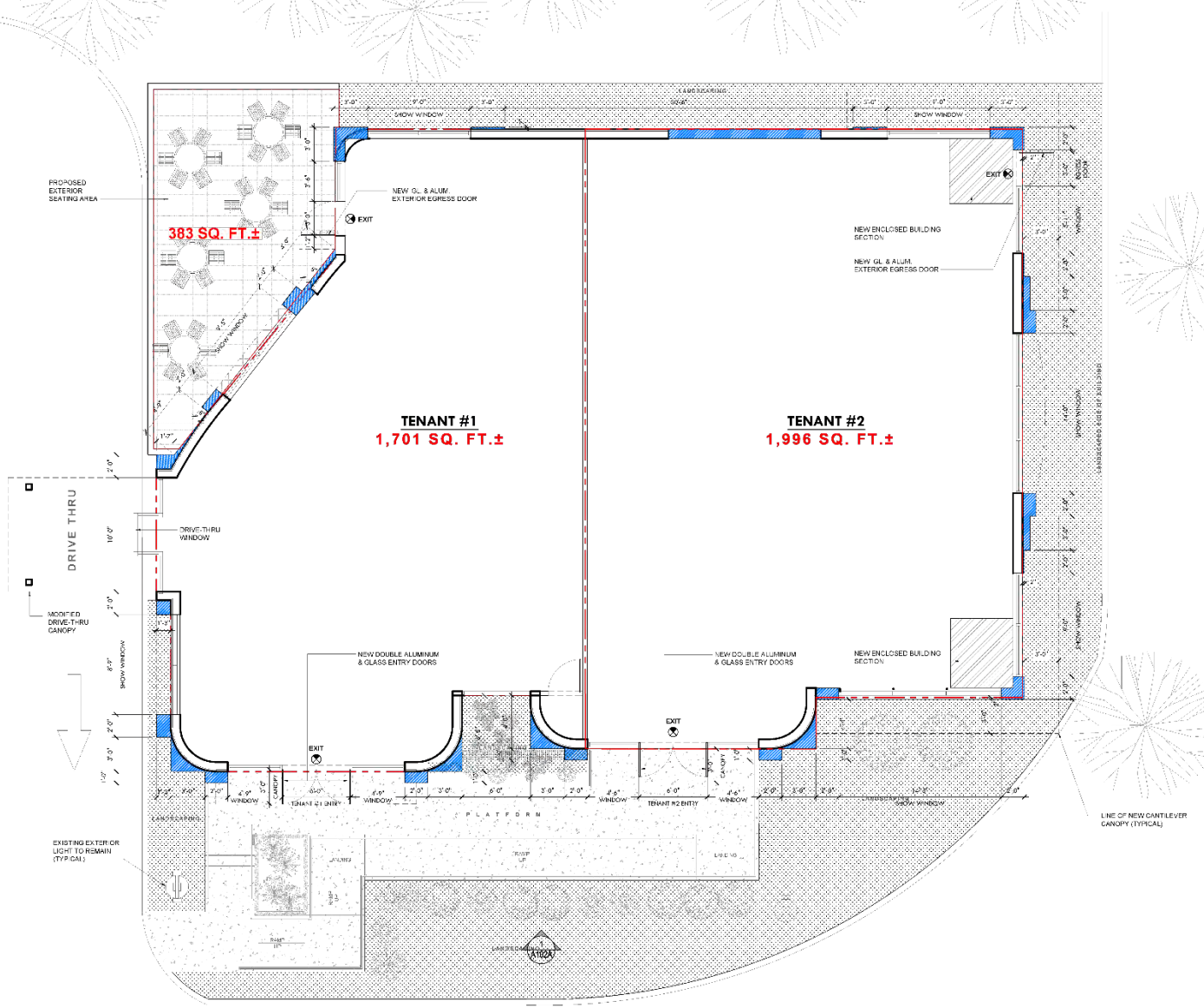
PROPOSED FLOOR PLAN '2' SCALE: 3/16" = 1'-0"
